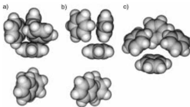
Figure 3. Space-filling representation of the principal phenyl–phenyl crystal contacts observed in a) benzene, b) peptide 2 , and c) peptides 1 and 3 .
