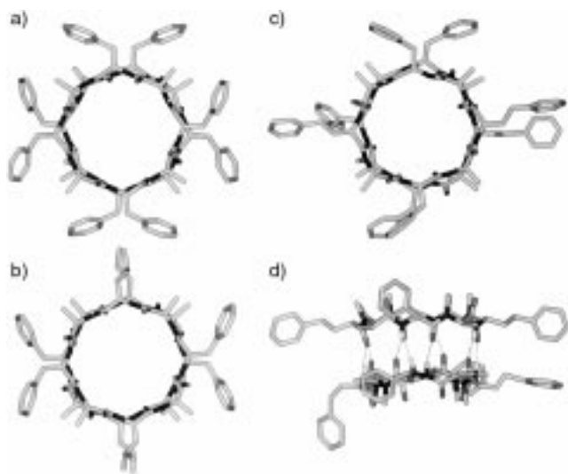
Figure 2. Crystal structures of dimeric \beta -sheet assemblies formed by a) cyclo [(-L-Phe-D-MeN-Ala) 4 -] ( 1 ); b) cyclo [(-L-Phe-D-MeN-Ala-L-Leu-D-MeN-Ala) 2 -] ( 3 ); c) cyclo [(-L-Phe-D-MeN-Ala-L-hPhe-D-MeN-Ala) 2 -] ( 2 ) viewed along the cylindrical axes, and d) across the dimeric interface of 2 .
