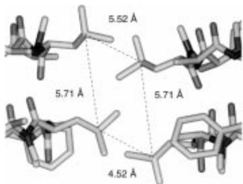
Figure 4. Stick representation of leucine-leucine interdimer lattice contacts in the crystal structure of 3 . Gamma-carbon distances are shown in Å.
